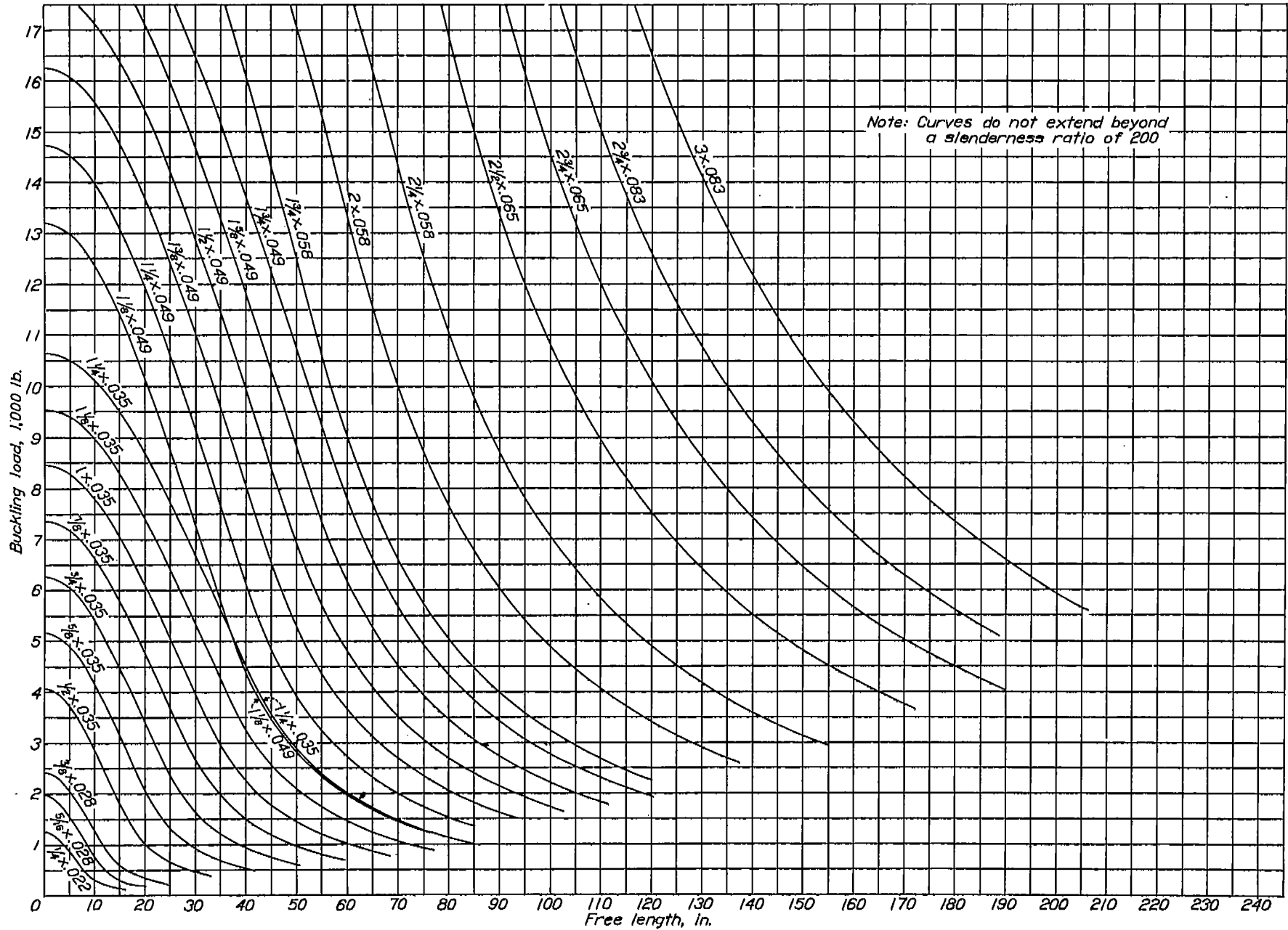
FIGURE 13.—The \sigma_c - P -diagram for Navy standard chromium-molybdenum-steel tubes. Y, S = 75,000 lb. per sq. in. E = 29,800,000 lb. per sq. in.
