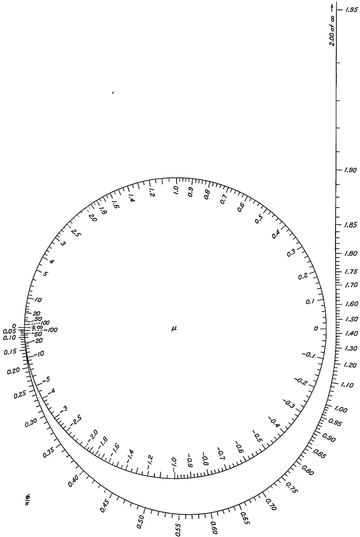
FIGURE 7.—Nomogram for determining \phi/\pi when two values of \mu are given.
