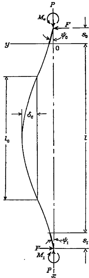
FIGURE 6.—Deflected center line of column.
