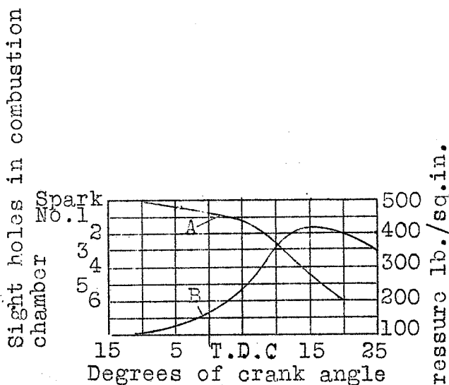
A, Curve of flame travel B, Pressure lb./sq.in. Fig. 4 Curves of observed spread of flame and pressure rise.
