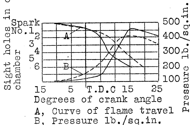
The curves shown in Figs. 4 & 5 superimposed. Fig. 6
