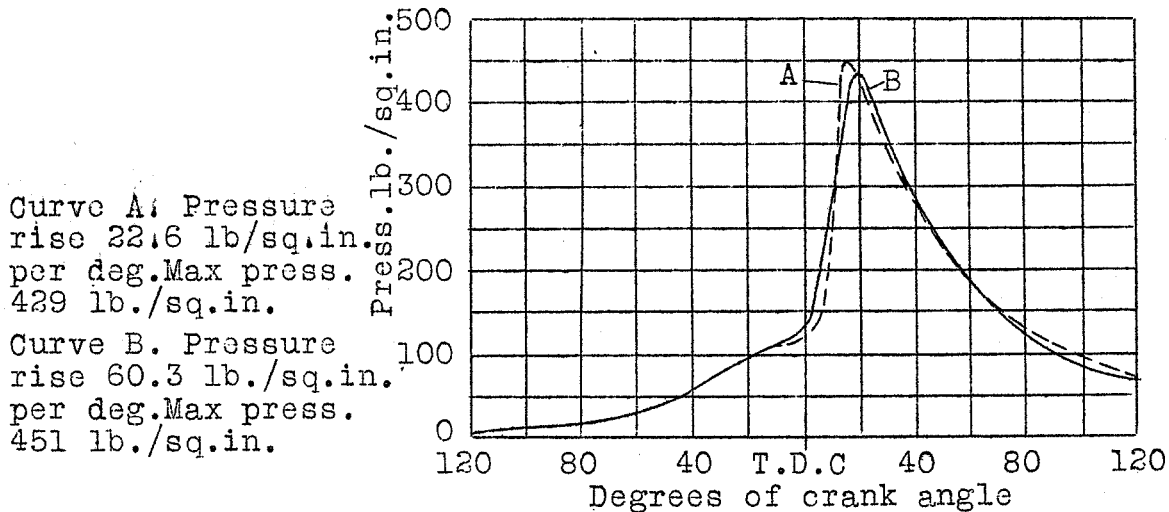
Fig.7 Two indicator diagrams showing normal and unduly rapid burning.
