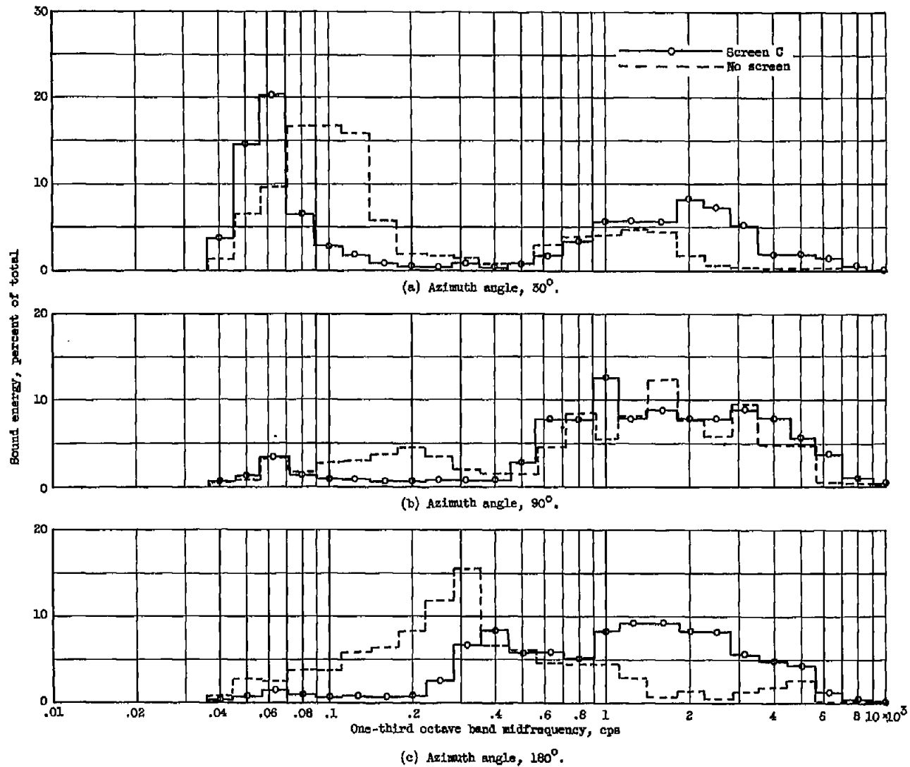
Figure 8. - Percentage of total sound energy in each one-third octave band for three points in sound field. Screen at minimum-power-level position.
