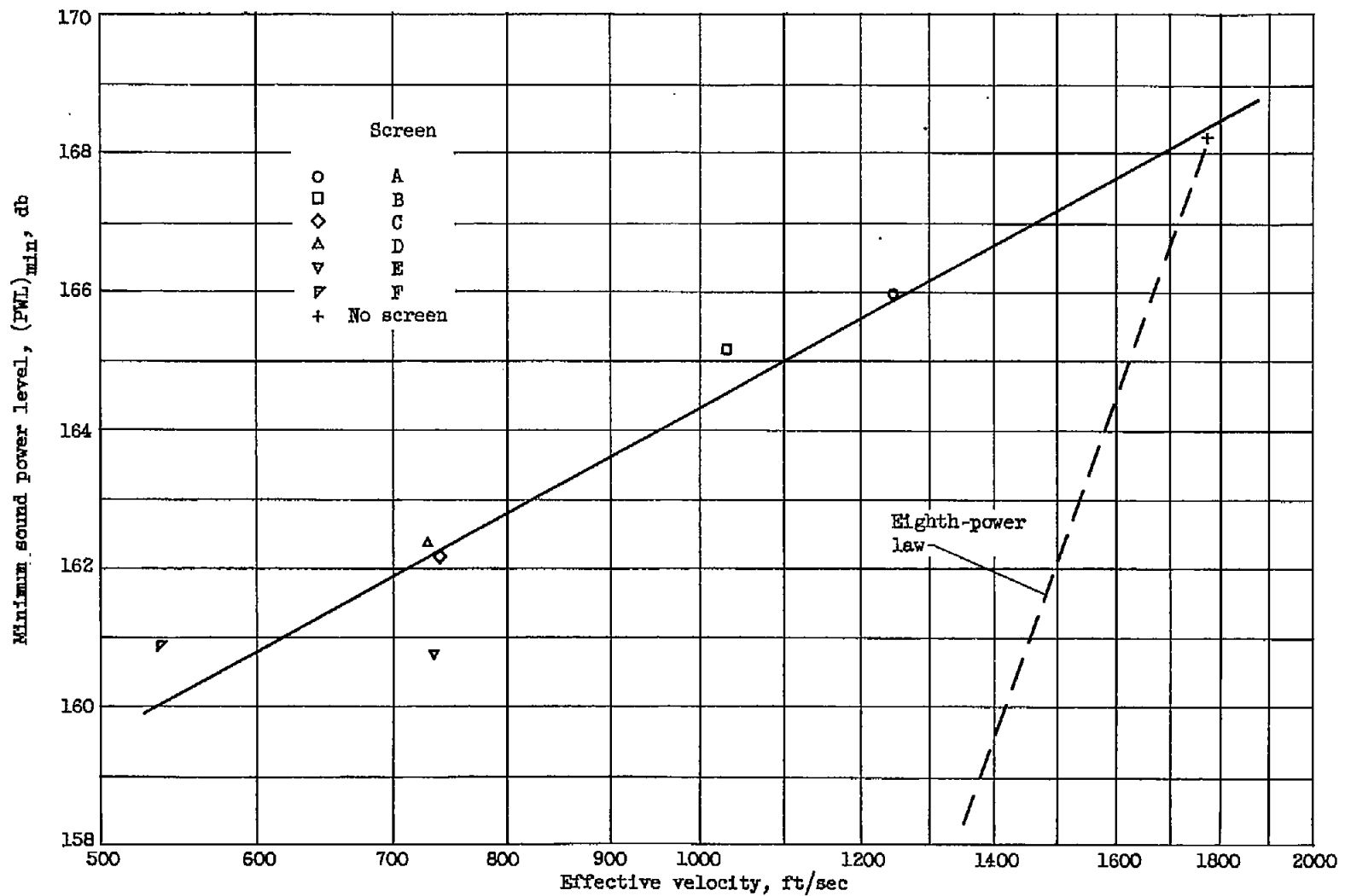
Figure 5. - Minimum sound power level at rated engine conditions as function of effective velocity.
