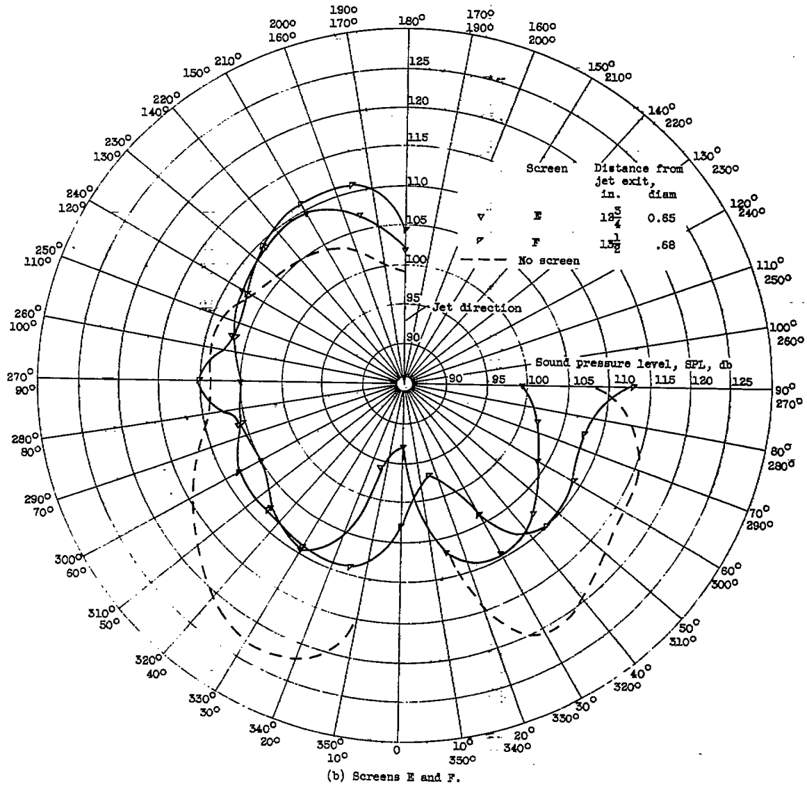
Figure 10. - Continued. Polar diagram of sound field at minimum-sound-power-level screen position. Distance from jet exit, 200 feet.
