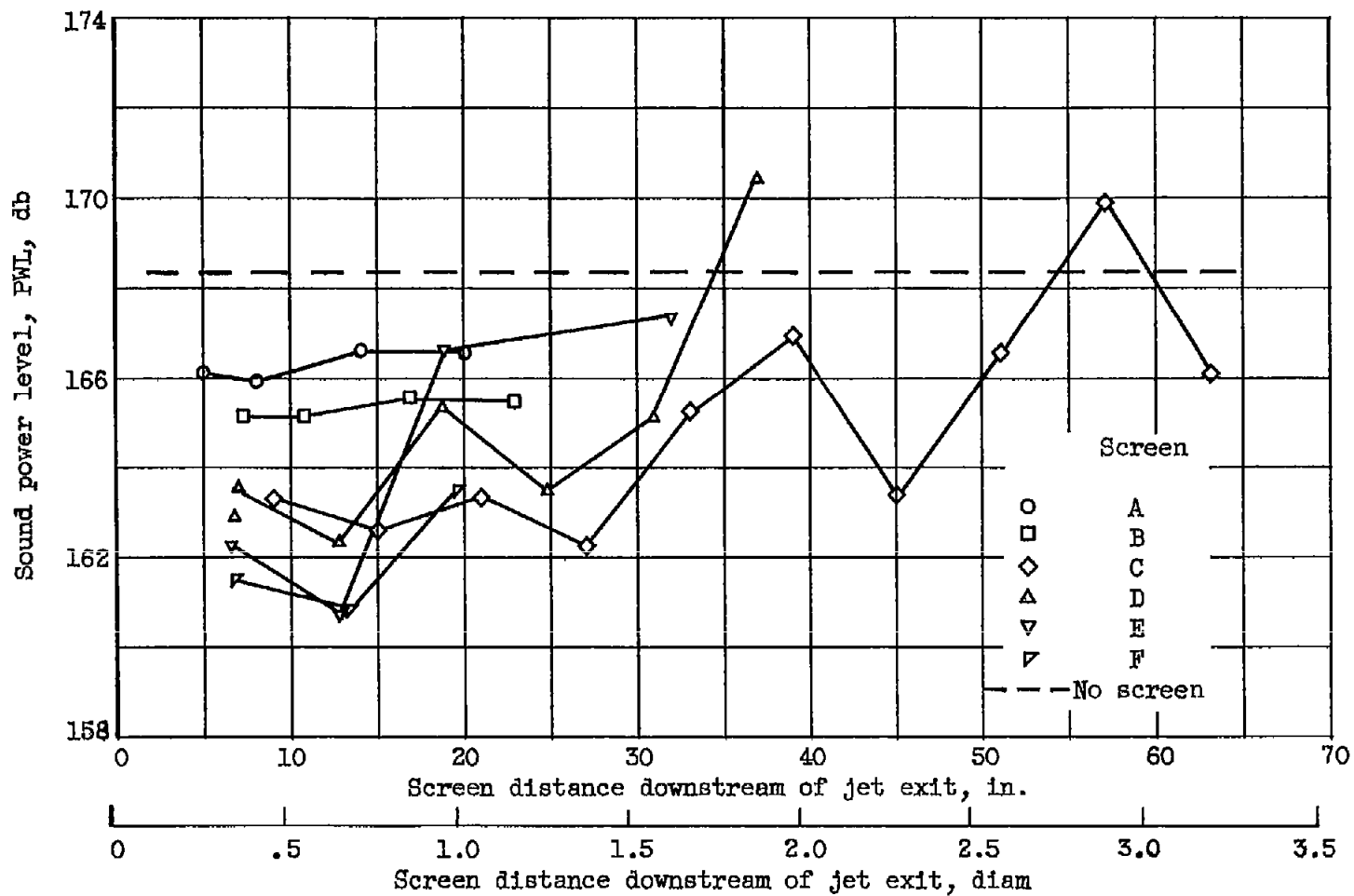
Figure 4. - Variation of sound power level as function of screen position for all screens investigated.
