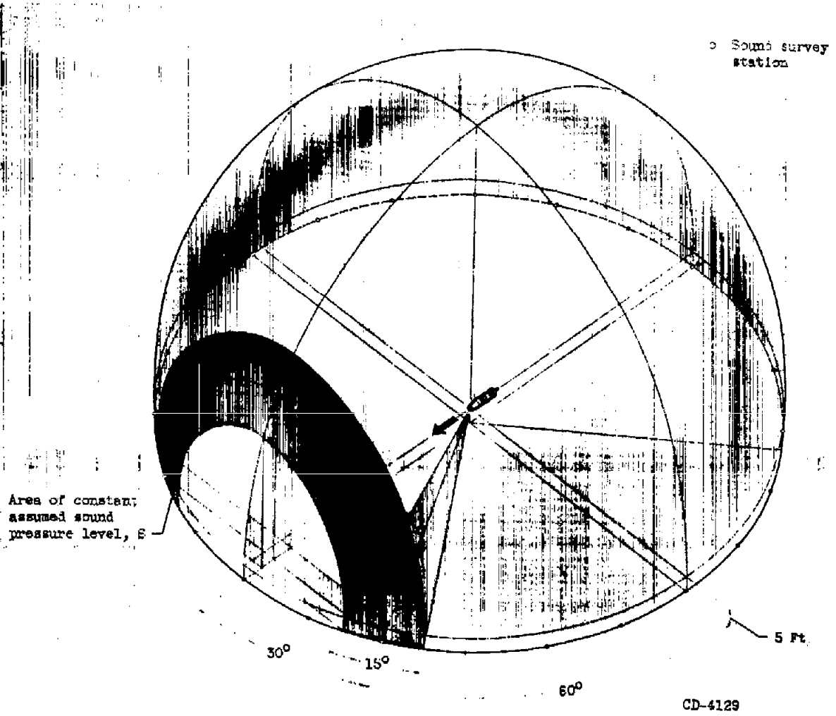
Figure 3. - Sketch illustrating surface used for calculation of sound power level radiated by engine.
