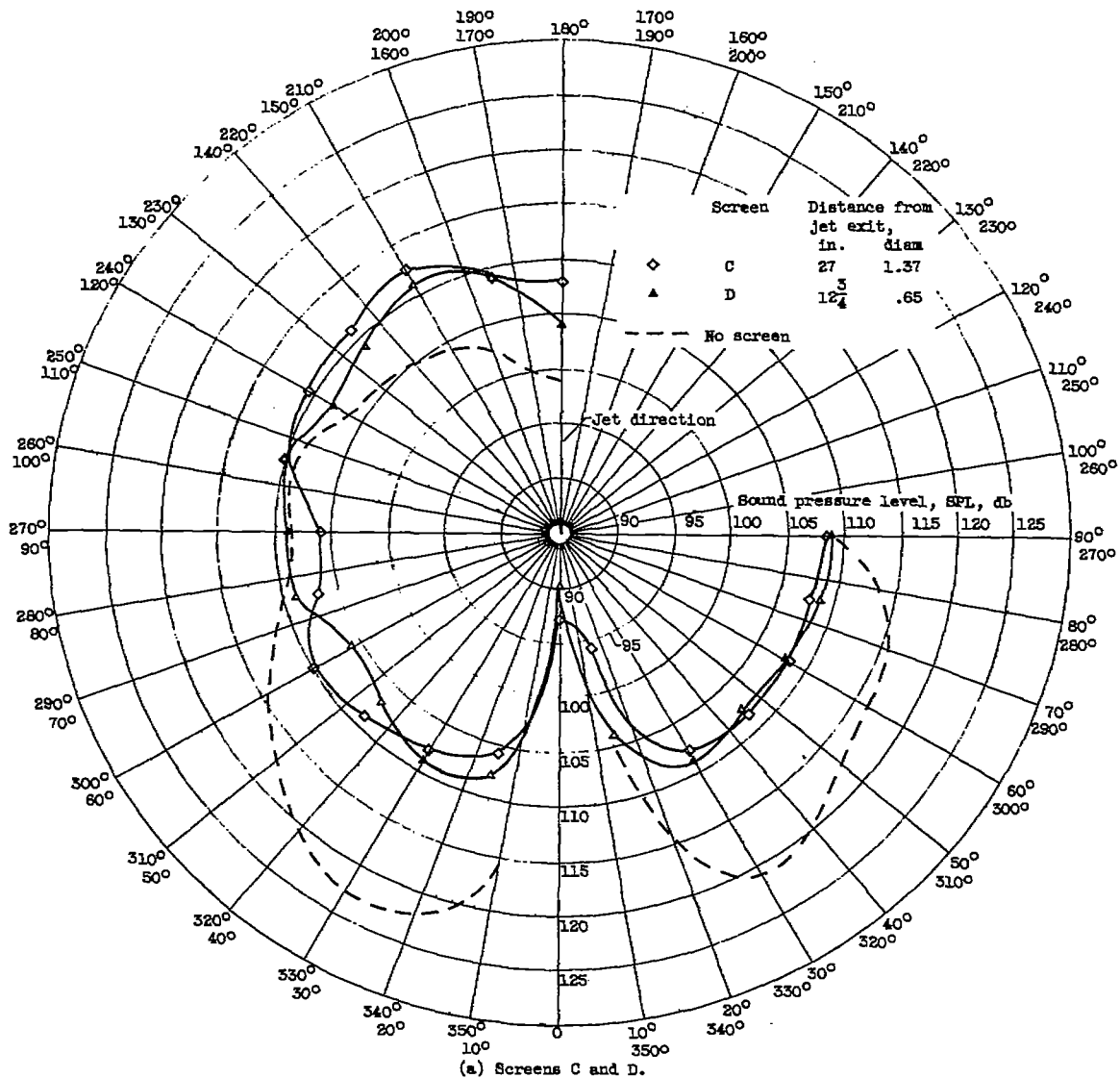
Figure 10. - Polar diagram of sound field at minimum-sound-power-level screen position. Distance from jet exit, 200 feet.
