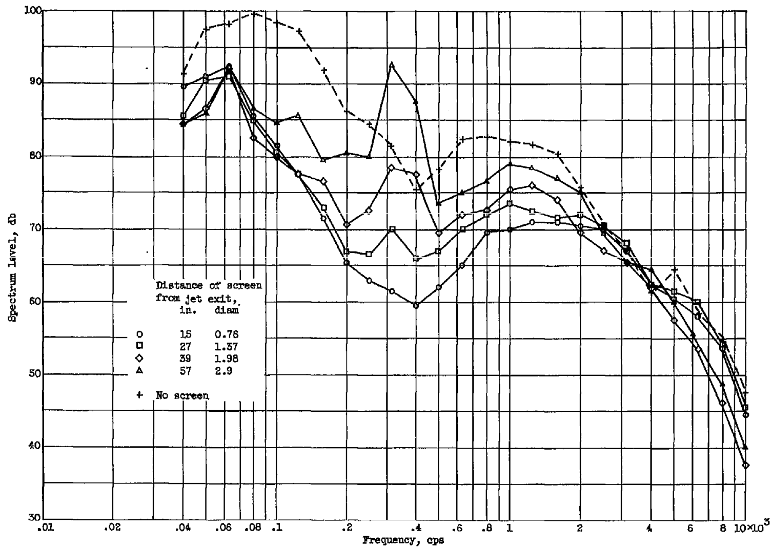
Figure 6. - Sound spectra of screen C for several screen positions. Distance from jet exit, 200 feet.
