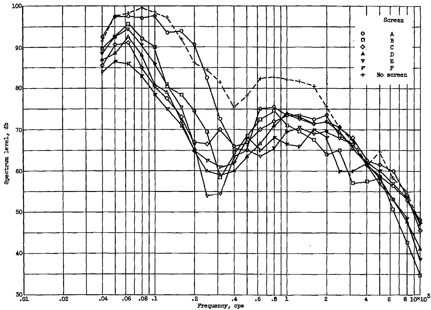
Figure 7. - Sound spectra at screen position of minimum sound power level for all screens. Distance from jet exit, 200 feet.
