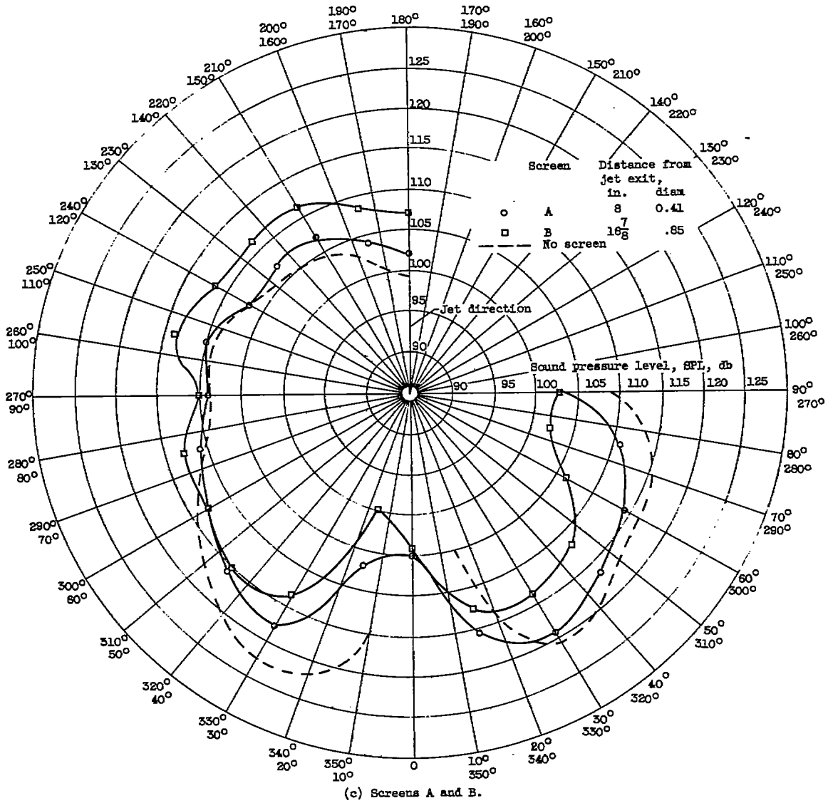
Figure 10. - Concluded. Polar diagram of sound field at minimum-sound-power-level screen position. Distance from jet exit, 200 feet.
