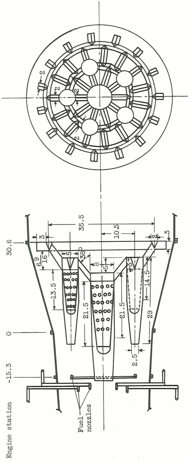
(a) Schematic diagram. (All dimensions in inches.)
