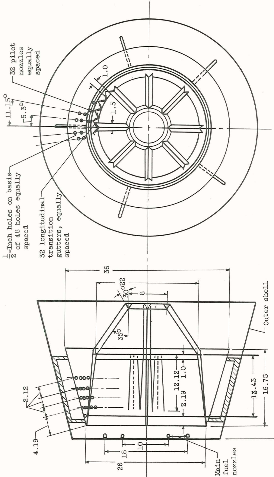
(a) Schematic diagram. (All dimensions in inches.)
