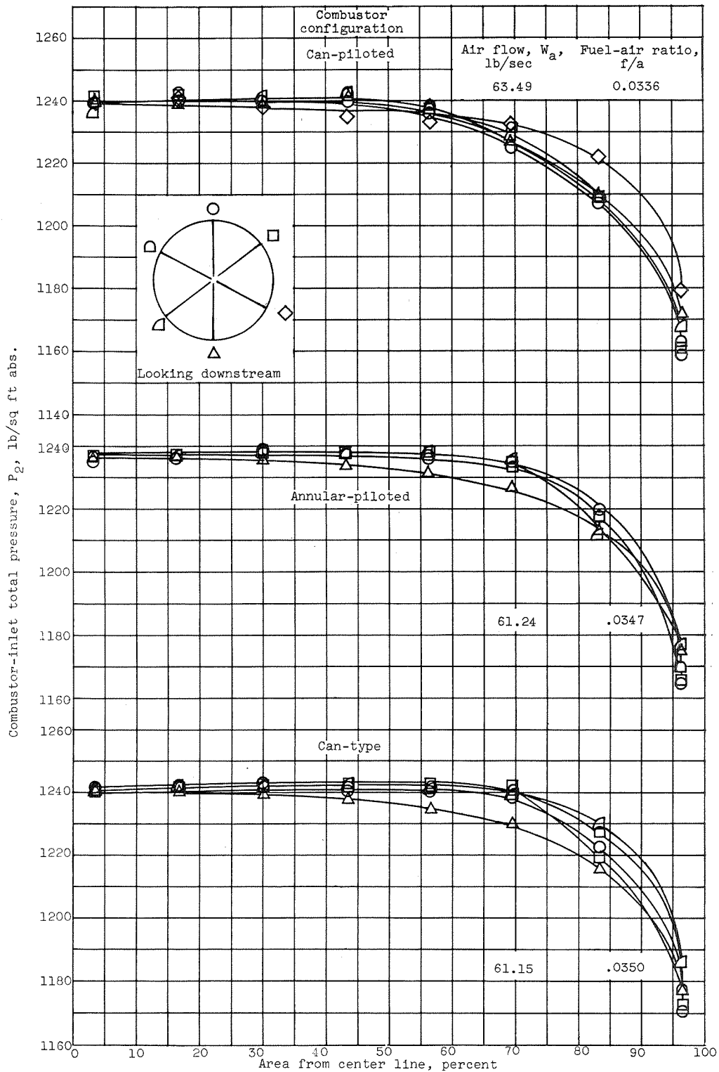
(a) Radial total-pressure distribution. Figure 6. - Combustor-inlet conditions for three low-temperature-ratio combustor configurations. Inlet-air temperature, 990° R.
